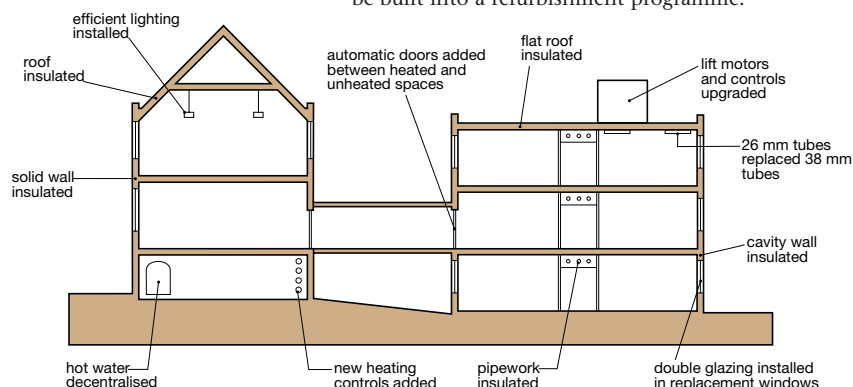
Figure 1 The opportunities for energy saving during refurbishment
